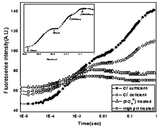
Fig. 2 The OJIP Chl a fluorescence transient curve (log time scale) in the PS II membranes of chloride-sufficient a , chloride-deficient b , chloride-depleted by sulphate c and chloride depleted by high pH d . Inset shows a characteristic OJIP curve shown with normal PS II membranes
